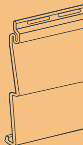
Double 5" Traditional Clapboard Exposure: 10" Length: 12'
