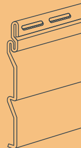
Double 4-1/2" Dutch Lap Exposure: 9" Length: 12' 1"
