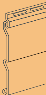
Double 5" Dutch Lap Exposure: 10" Length: 12'
