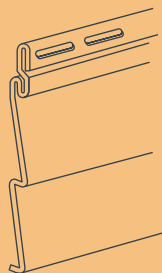
Double 4" Traditional Clapboard Exposure: 8" Length: 12' 6"
