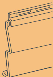
Double 4" Traditional Clapboard Exposure: 8" Length: 12' 6"
