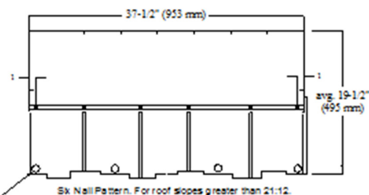
FIGURE 1—SHINGLE PROFILES AND FASTENER PATTERNS (Continued)
